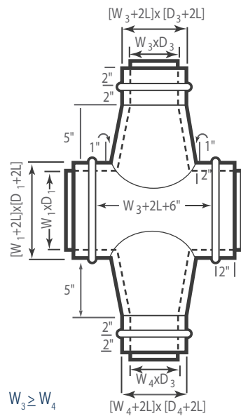
Conical Cross
