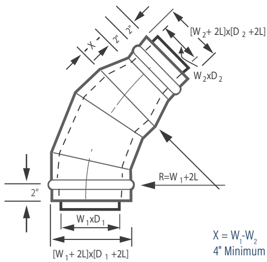
45° 3-Piece Elbow with Reducer
