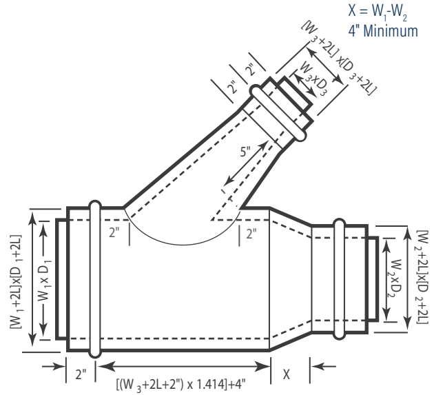
Reducing Conical Lateral 45°
