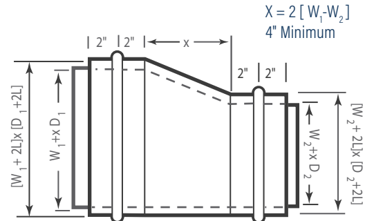
Eccentric Reducer
