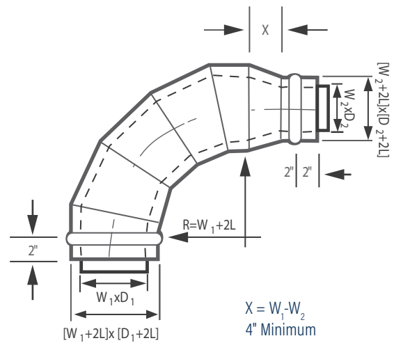
90° 5-Piece Elbow with Reducer
