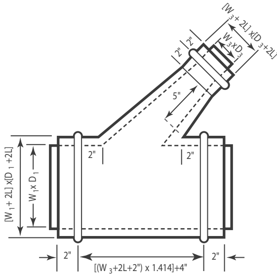
Conical Lateral 45°
