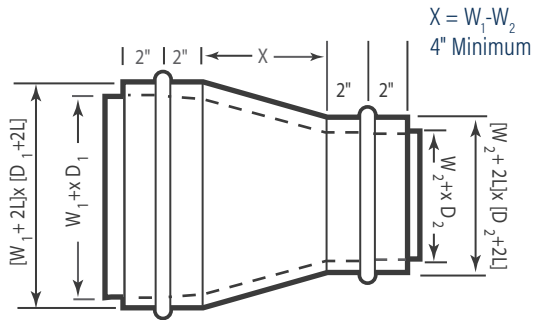
Concentric Reducer
