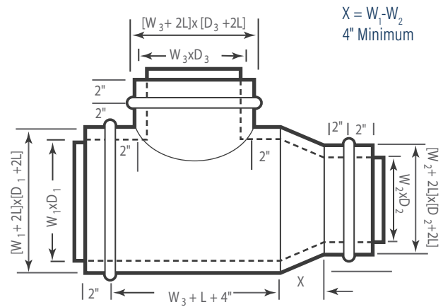
Reducing Tee
