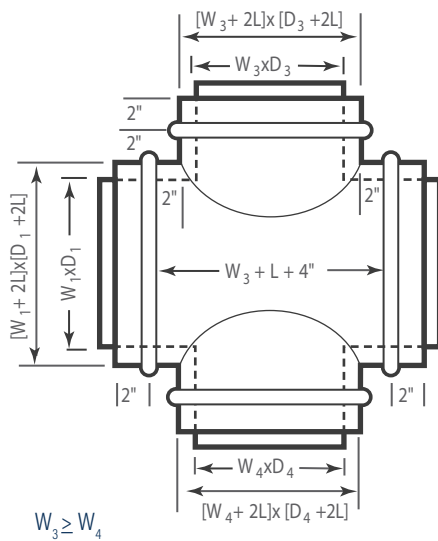
Cross Tee
