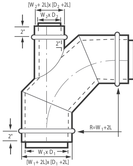
90° 3-Piece Elbow with Heel Tap
