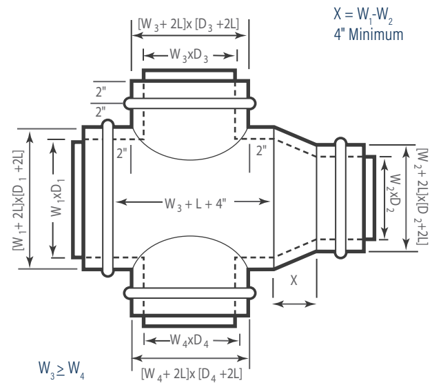
Reducing Cross Tee
