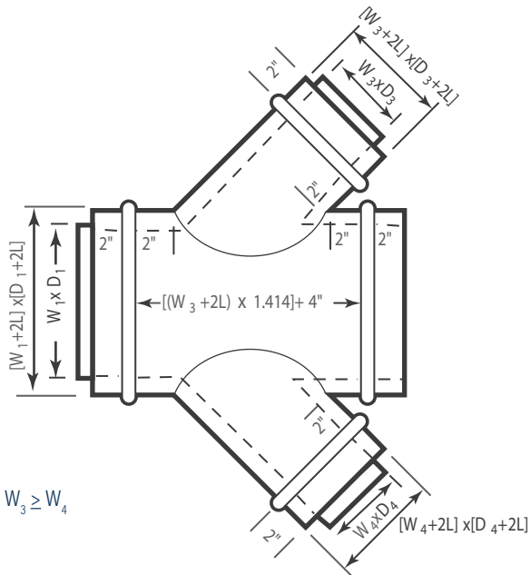
Lateral Cross 45°
