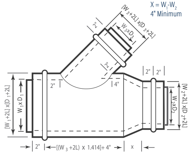
Reducing Lateral 45°
