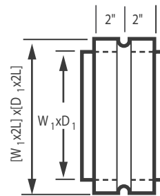
Fitting Couplings
