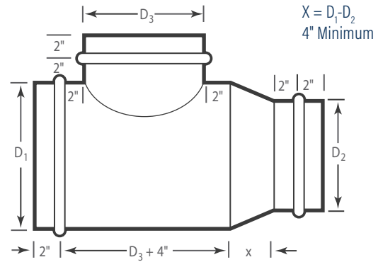
Reducing Tee
