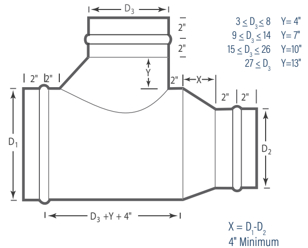
Reducing Combination Tee
