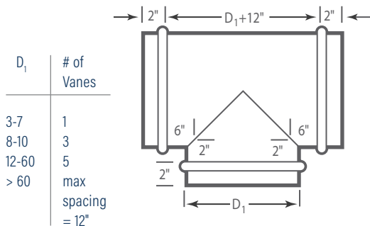
Bullhead Tee
