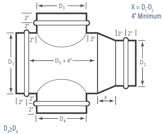
Reducing Cross Tee
