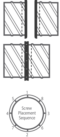
Installation of Flange Connector
