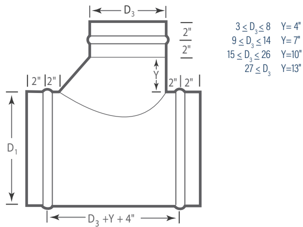
Combination Tee
