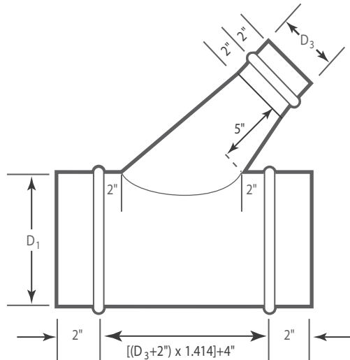
Conical Lateral 45°
