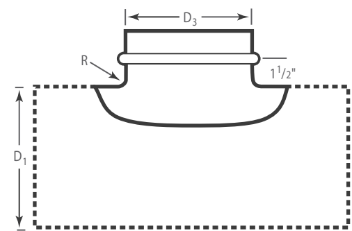
Field Installed Pressed Tap
