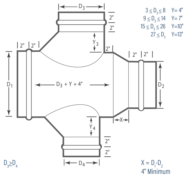
Reducing Combination Cross
