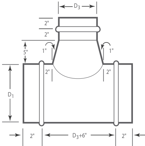
Conical Tee
