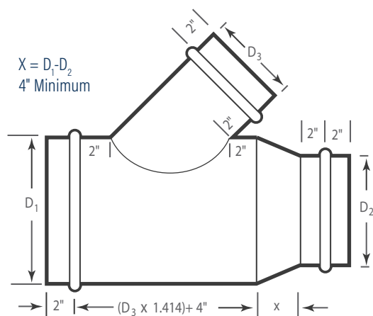
Reducing Lateral 45°
