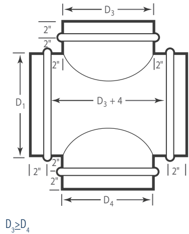
Cross Tee
