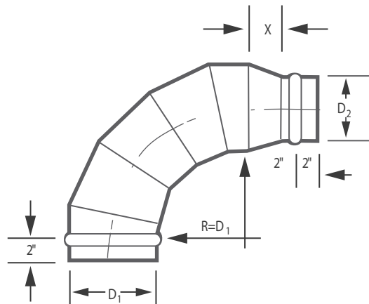
90° 5-Piece Elbow with Reducer
