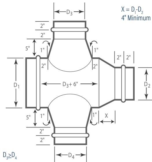
Reducing Conical Cross Tee
