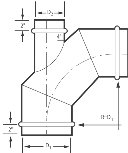
90° 3-Piece Elbow with Heel Tap
