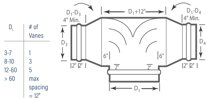
Reducing Bullhead Tee
