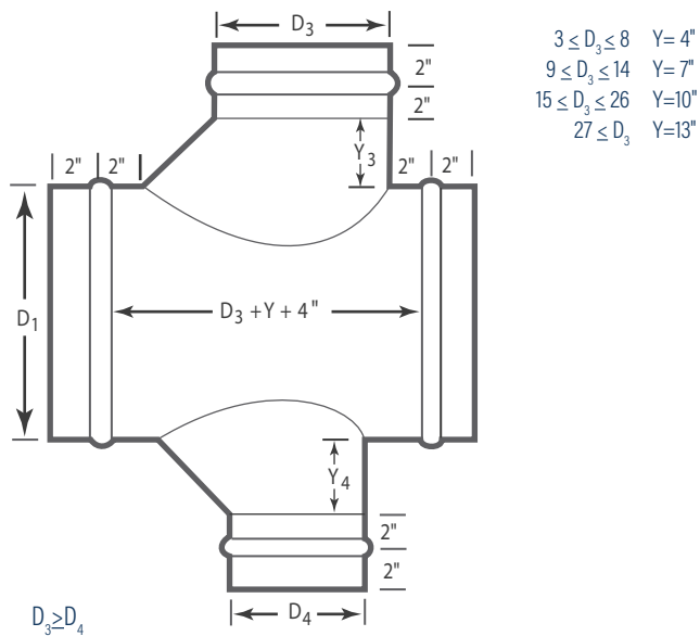
Combination Cross
