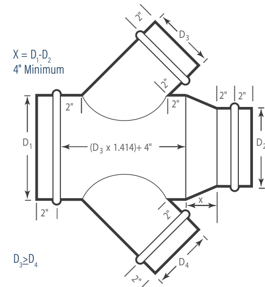
Reducing 45° Lateral Cross
