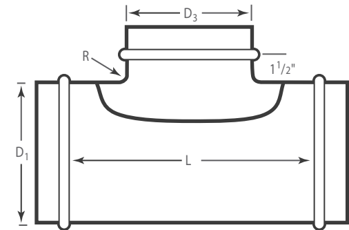
Pressed Tee
